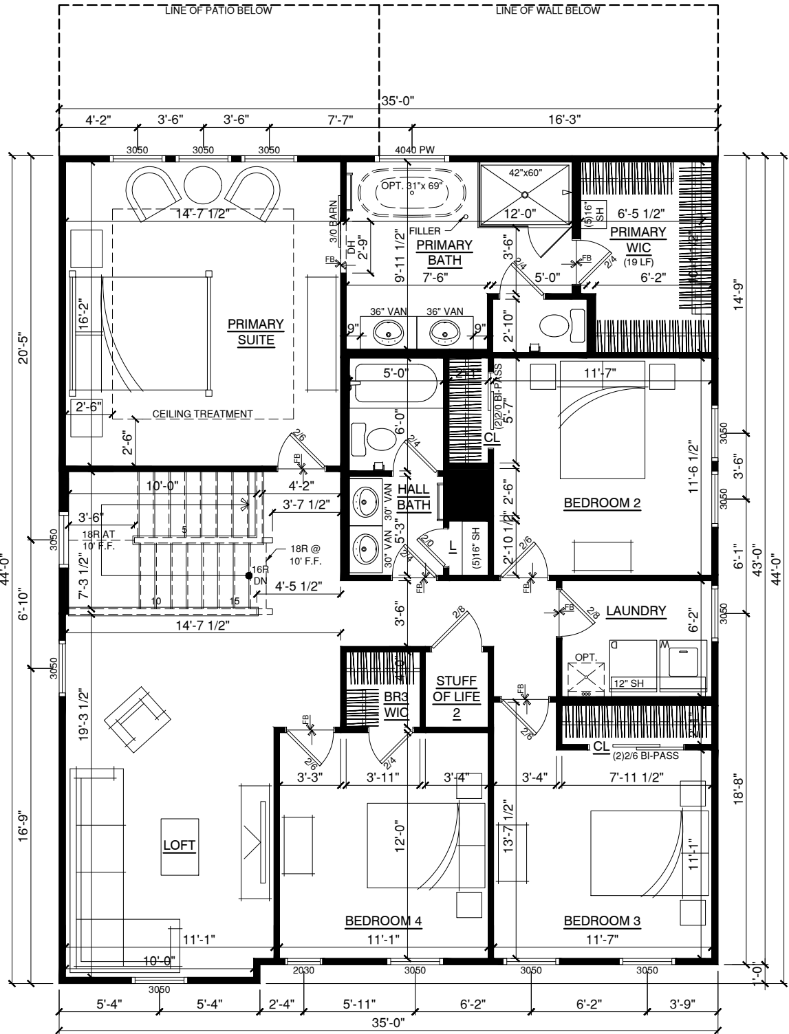
SECOND FLOOR
