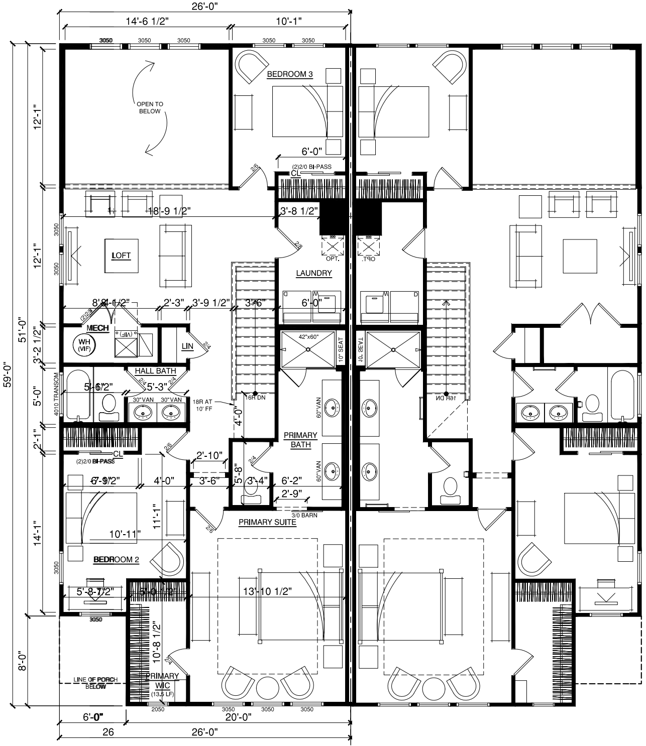
SECOND FLOOR
