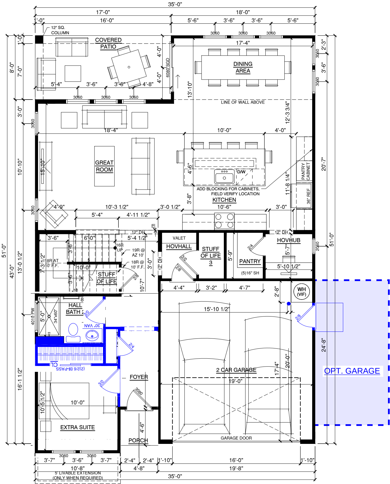
FIRST FLOOR
