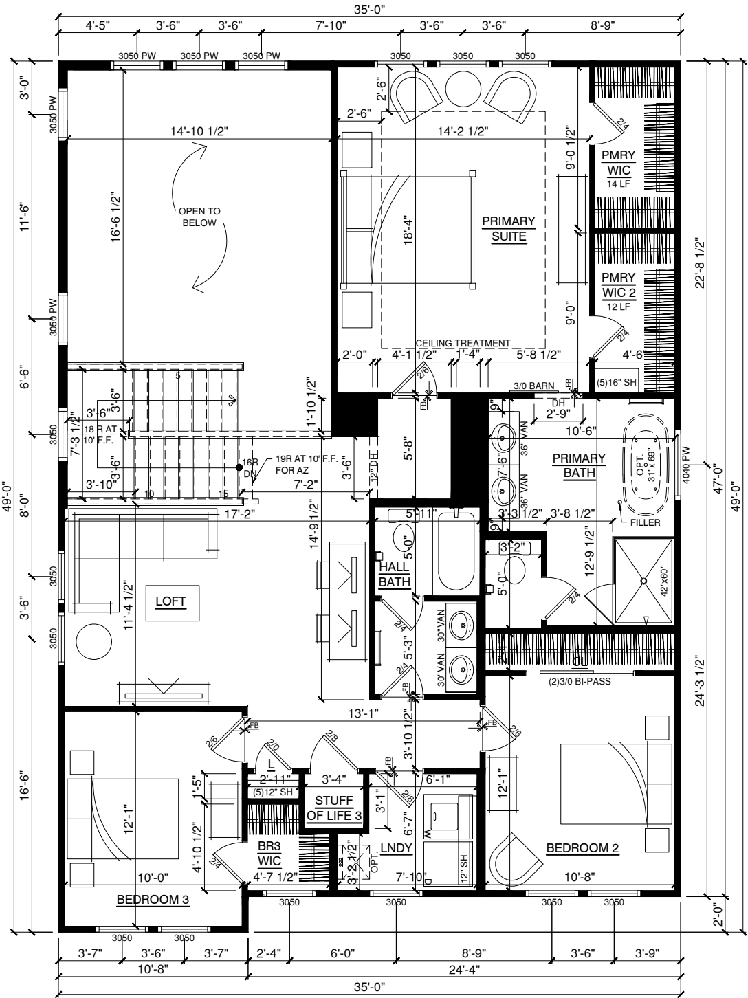
SECOND FLOOR
