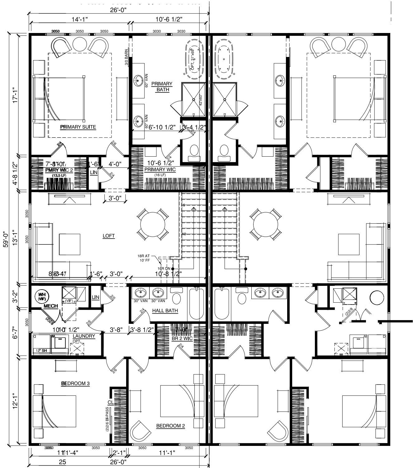
SECOND FLOOR
