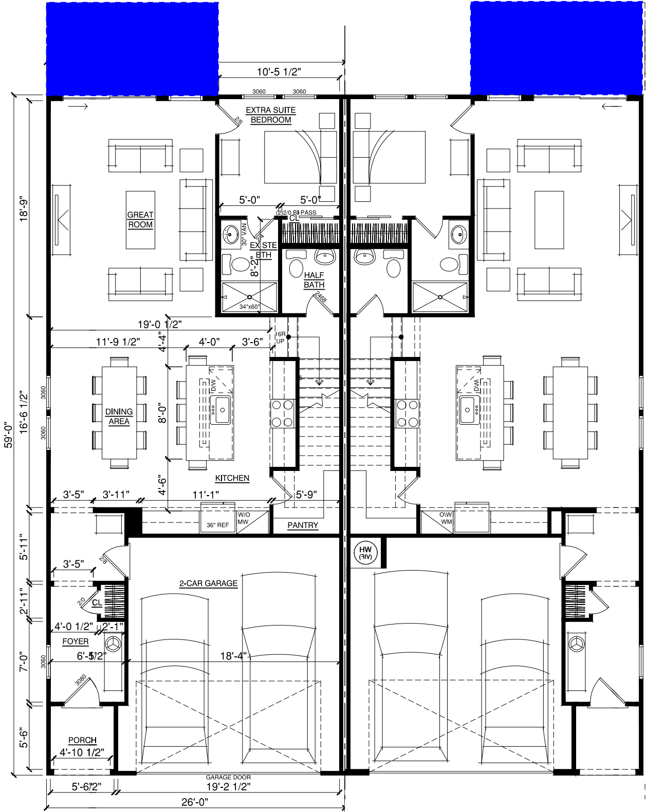
FIRST FLOOR
