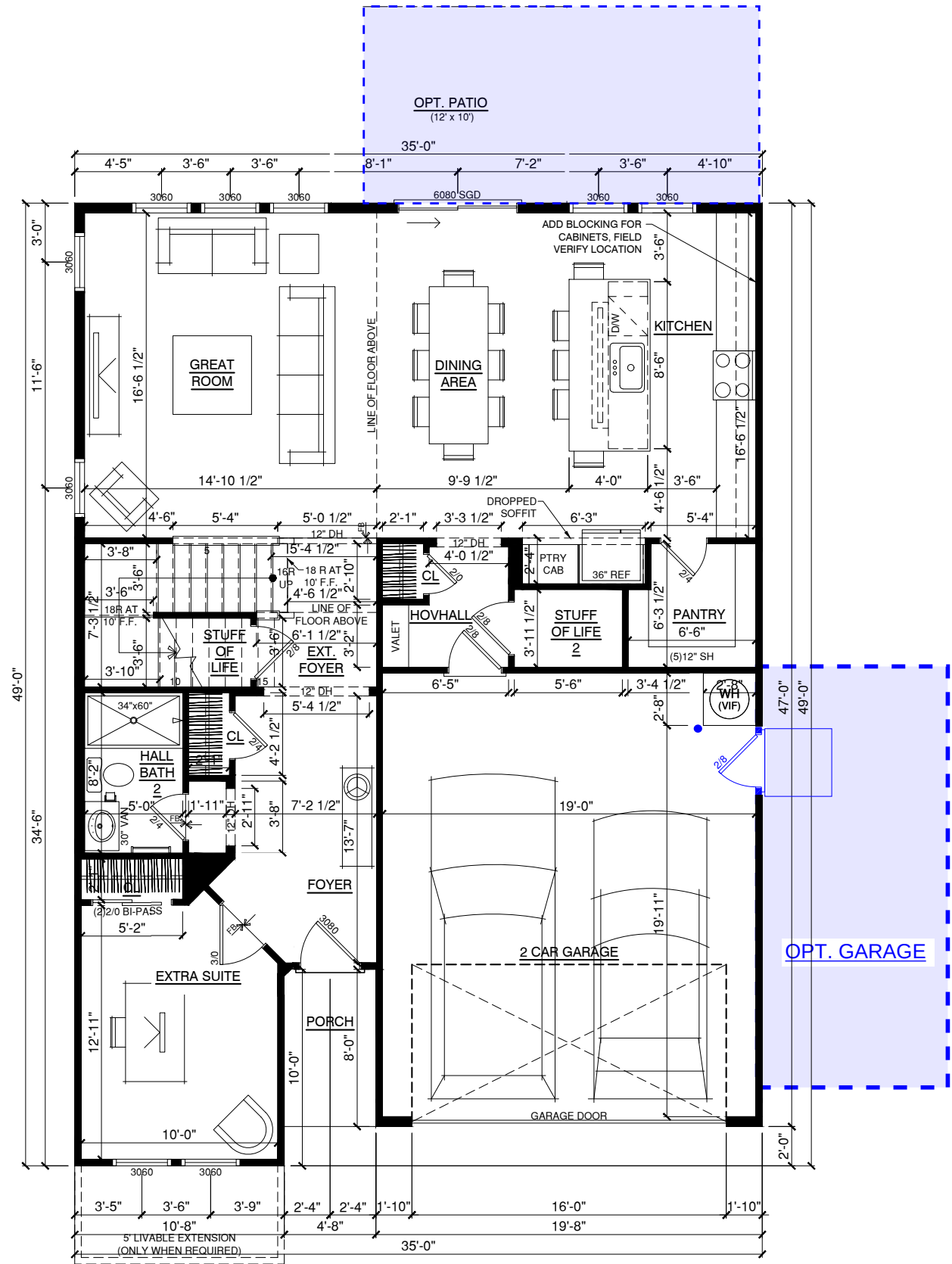
FIRST FLOOR
