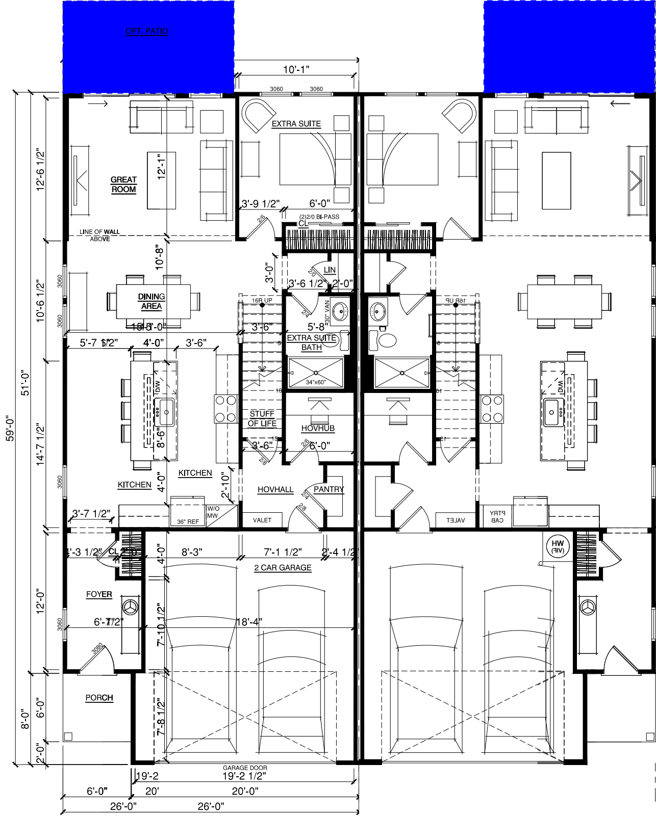
FIRST FLOOR
