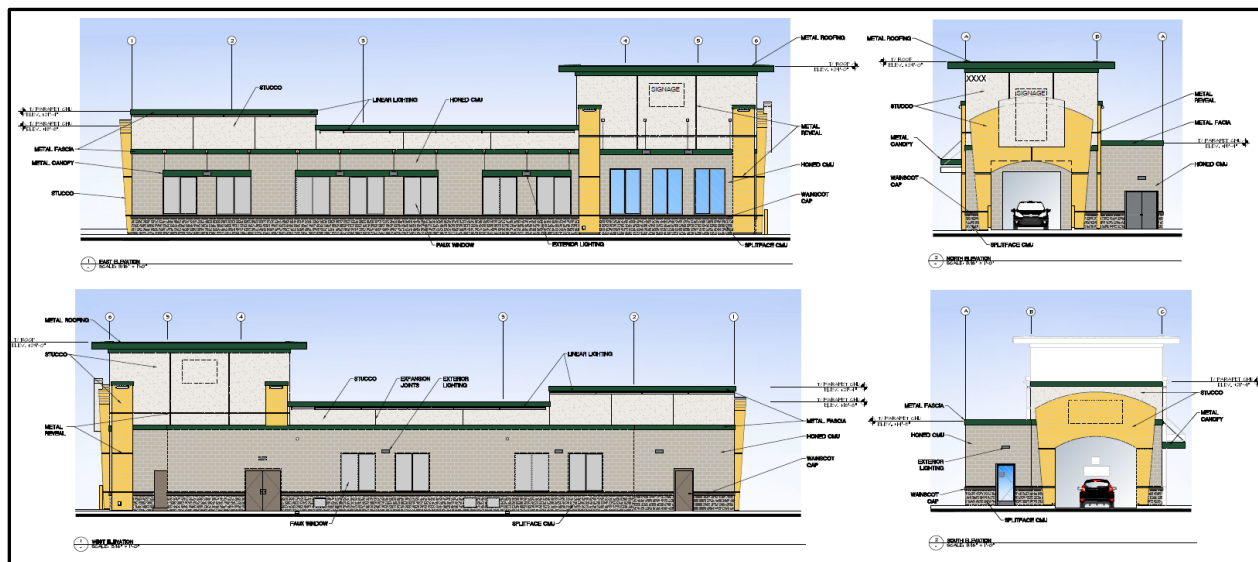
Figure 3a: Elevations of proposed Quick Quack carwash
