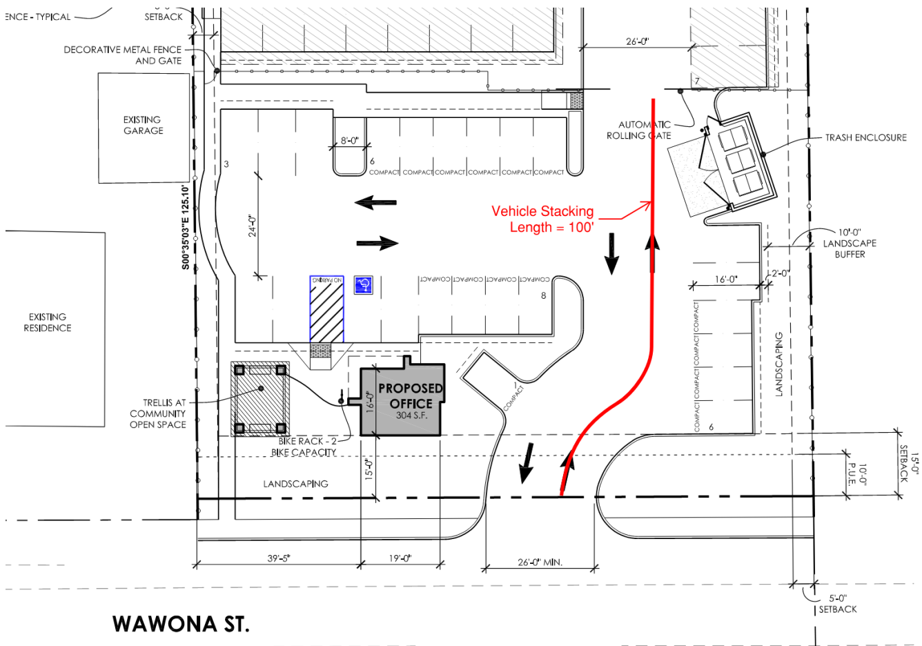
Figure 8. Project Gate Stacking Length
