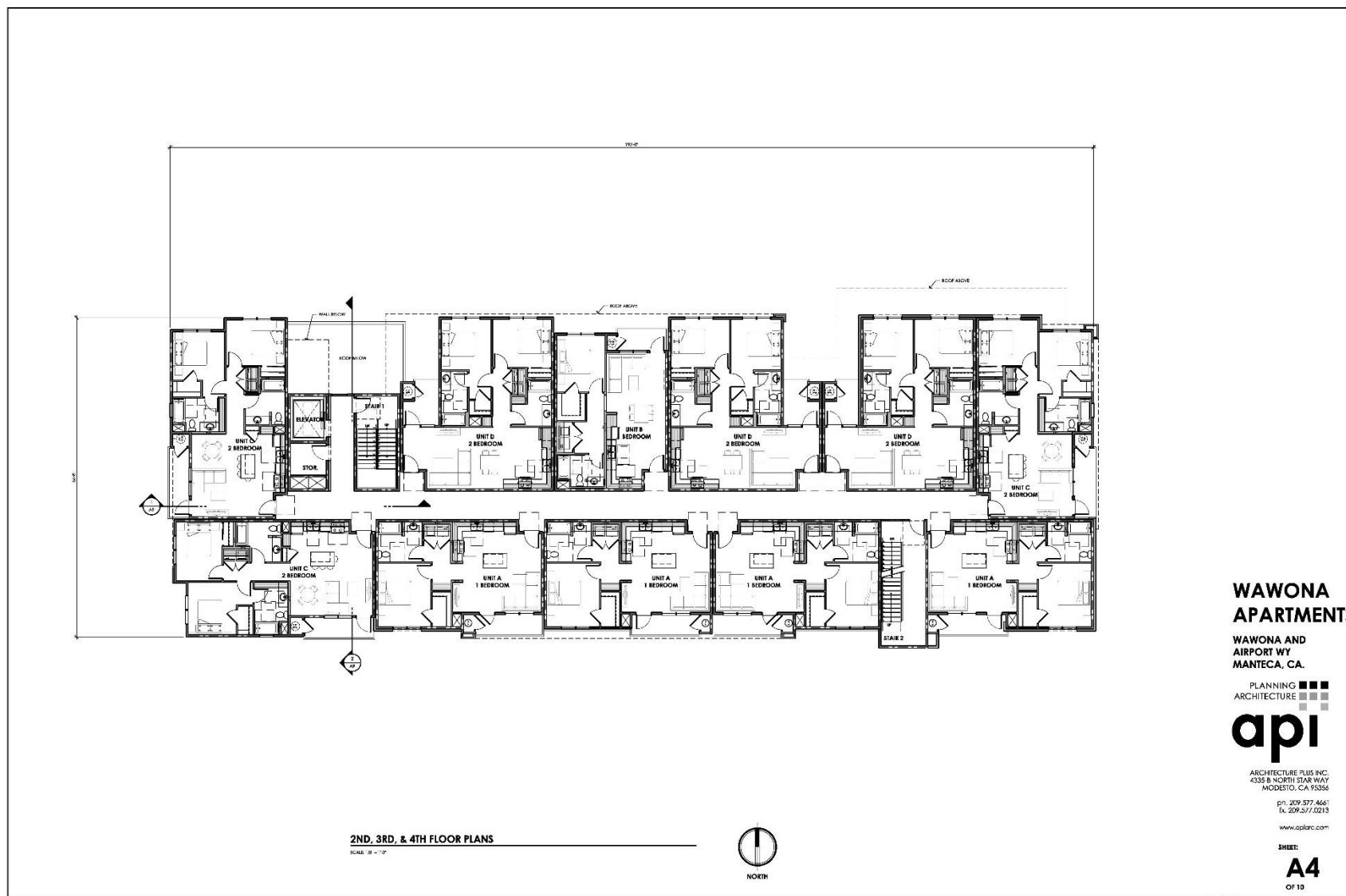
Figure 2-10 2nd, 3rd, and 4th Floor Plan
